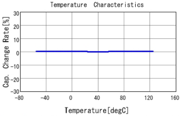
GRM1555C1H1R5BA01 C-Temp. capchange, DC0V, AC1Vrms
