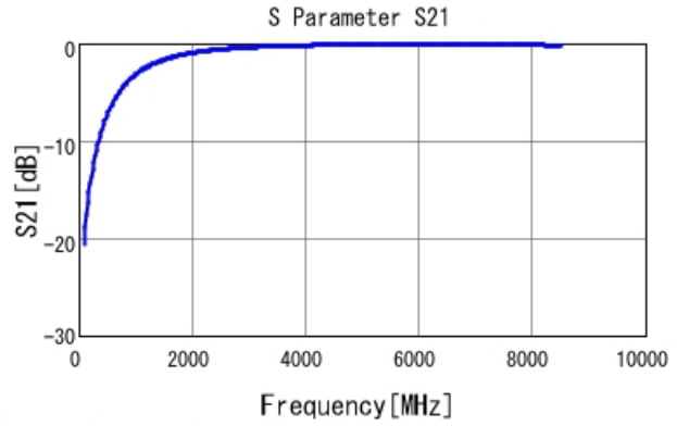
GRM1555C1H1R5BA01 S21 DC0V, 25degC
