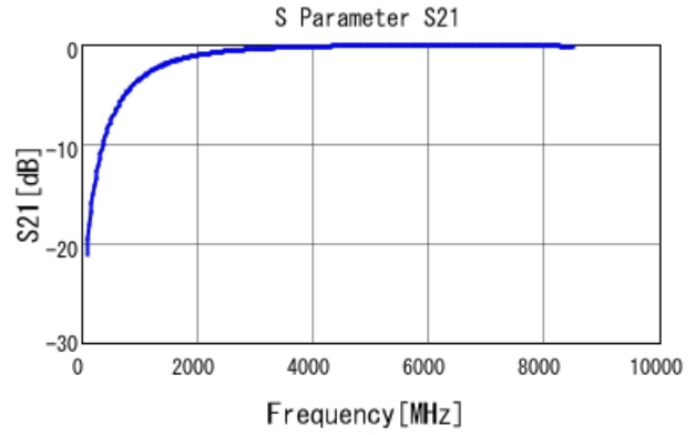
GRM1555C1H1R4WA01 S21 DC0V, 25degC
