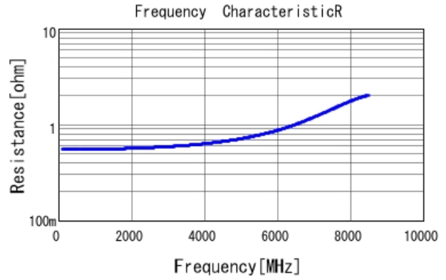
GRM1555C1H1R4WA01 R DCOV, 25degC
