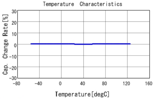
GRM1555C1H1R4WA01 C-Temp. capchange, DC0V, AC1Vrms
