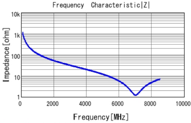
GRM1555C1H1R4WA01 |Z| DCOV, 25degC
