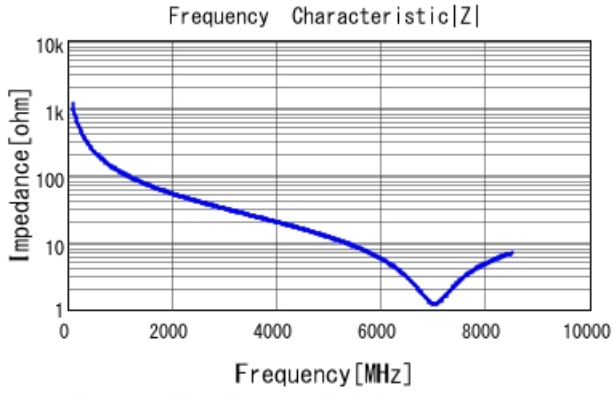
GRM1555C1H1R4BA01 |Z| DCOV, 25degC
