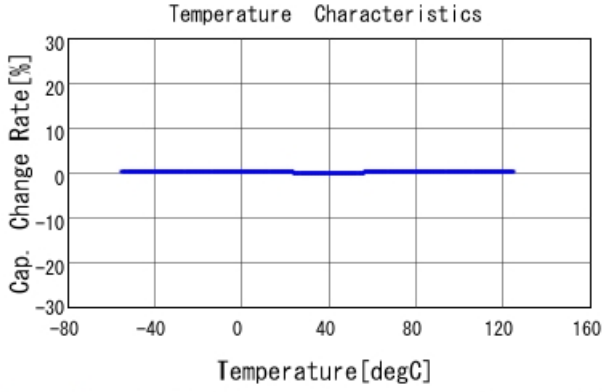
GRM1555C1H1R4BA01 C-Temp. capchange, DC0V, AC1Vrms
