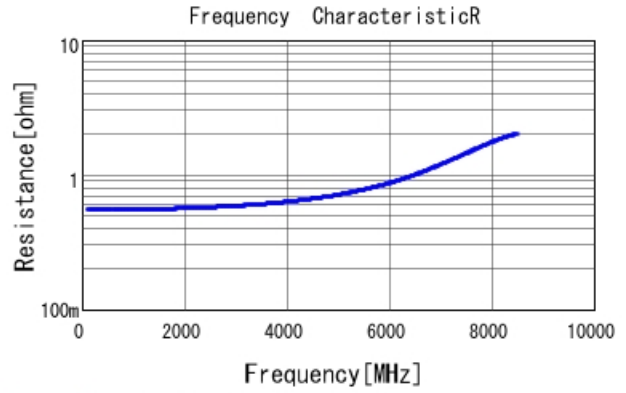
GRM1555C1H1R4BA01 R DCOV, 25degC
