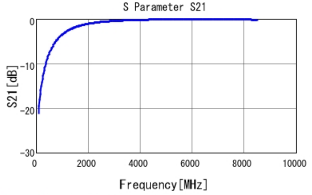
GRM1555C1H1R4BA01 S21 DC0V, 25degC
