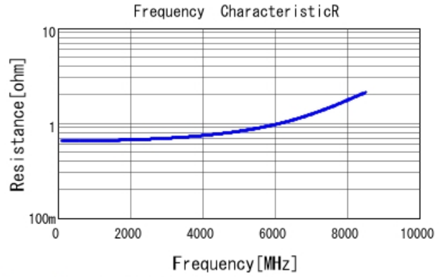
GRM1555C1H1R3BA01 R DCOV, 25degC
