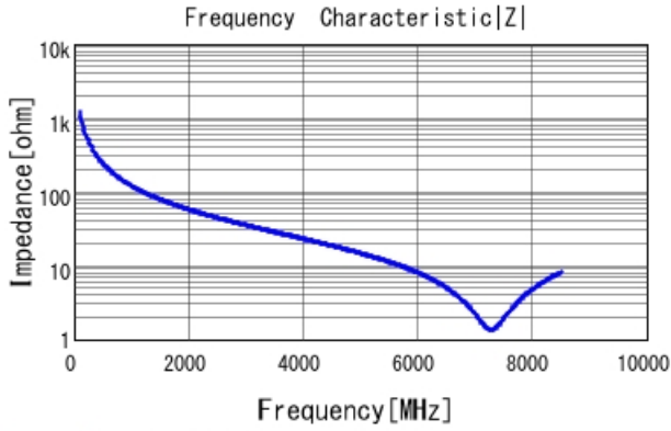
GRM1555C1H1R3BA01 |Z| DCOV, 25degC
