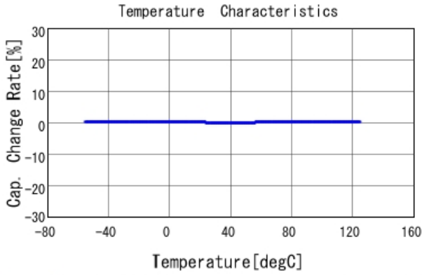
GRM1555C1H1R3BA01 C-Temp. capchange, DC0V, AC1Vrms
