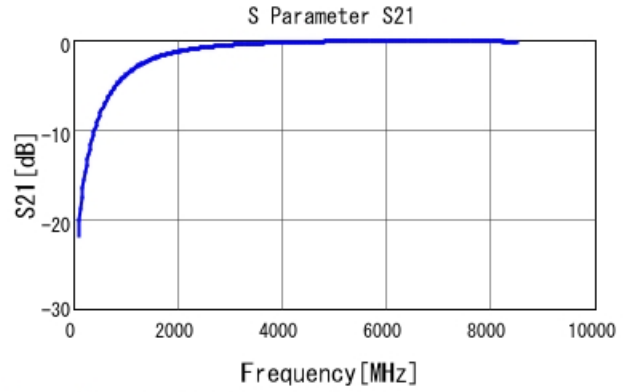
GRM1555C1H1R3BA01 S21 DC0V, 25degC
