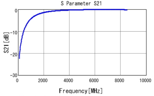
GRM1555C1H1R2CA01 S21 DCOV, 25degC
