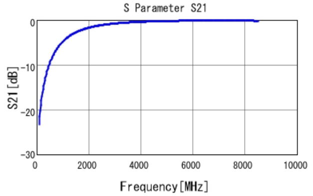
GRM1555C1H1R1WA01 S21 DCOV, 25degC
