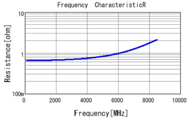
GRM1555C1H1R1WA01 R DCOV, 25degC
