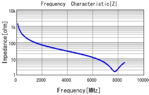
GRM1555C1H1R1WA01 |Z| DCOV, 25degC
