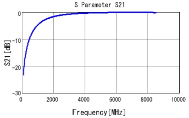
GRM1555C1H1R1CA01 S21 DCOV, 25degC
