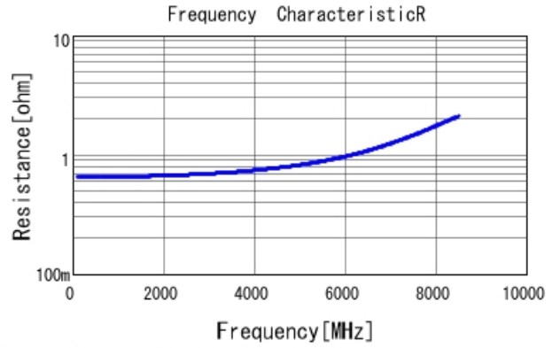
GRM1555C1H1R1CA01 R DCOV, 25degC
