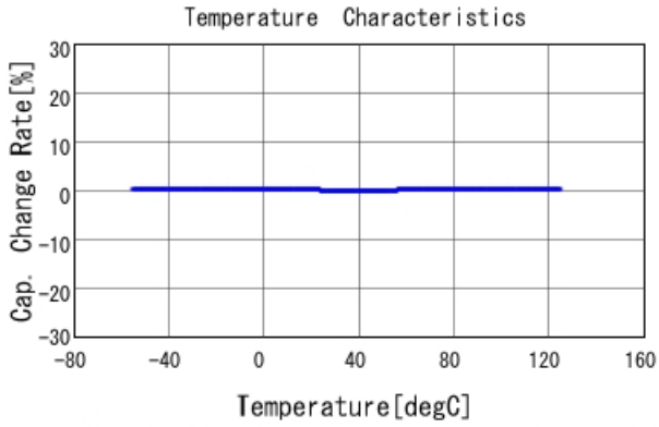
GRM1555C1H1R1CA01 C-Temp. capchange, DCOV, AC1Vrms
