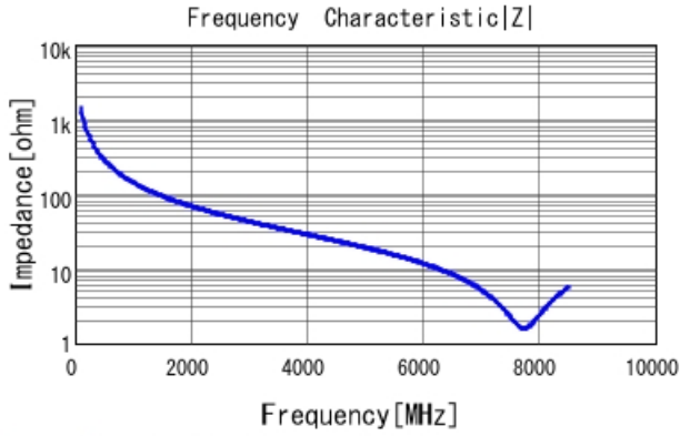
GRM1555C1H1R1CA01 |Z| DCOV, 25degC
