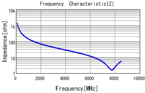
GRM1555C1H1R1BA01 |Z| DCOV, 25degC
