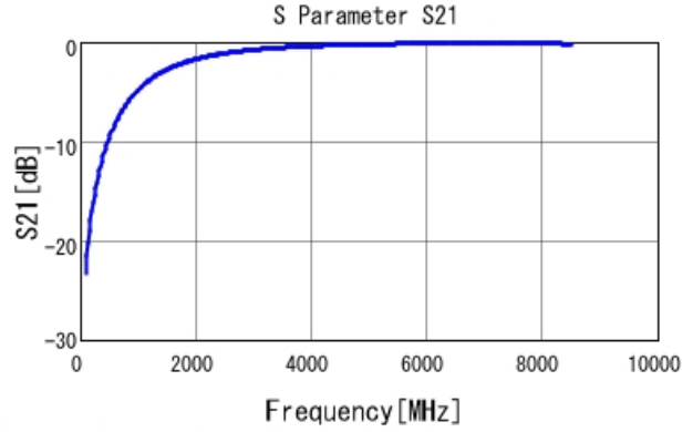
GRM1555C1H1R1BA01 S21 DCOV, 25degC
