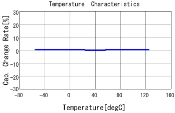
GRM1555C1H1R1BA01 C-Temp. capchange, DCOV, AC1Vrms
