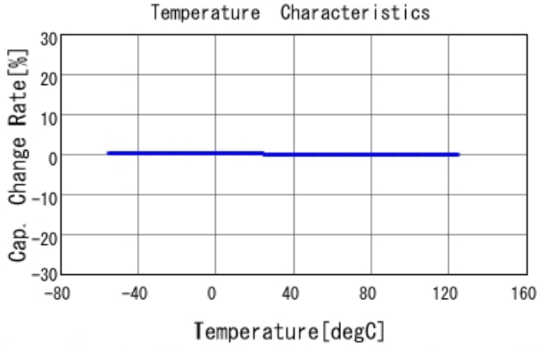
GRM1555C1H182JA01 C-Temp. capchange, DCOV, AC1Vrms
