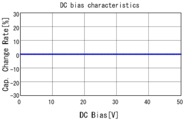
GRM1555C1H182GA01 C-DC bias capchange, 25.0degC, A
