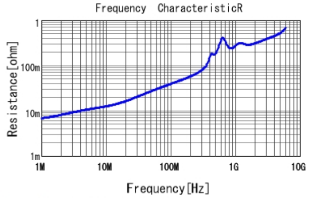
GRM1555C1H182GA01 R DCOV, 25degC
