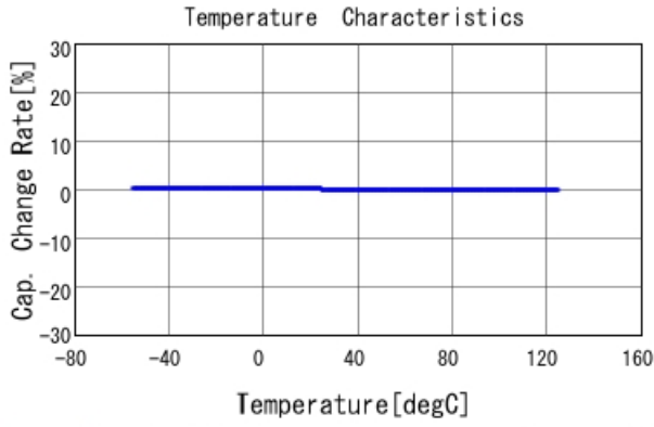
GRM1555C1H182GA01 C-Temp. capchange, DCOV, AC1Vrms
