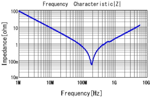
GRM1555C1H182GA01 |Z| DCOV, 25degC
