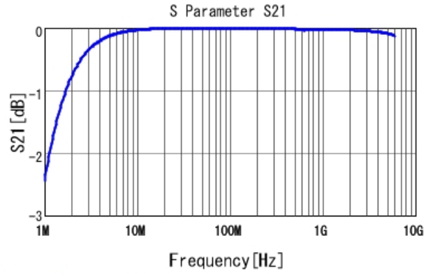
GRM1555C1H182GA01 S21 DCOV, 25degC
