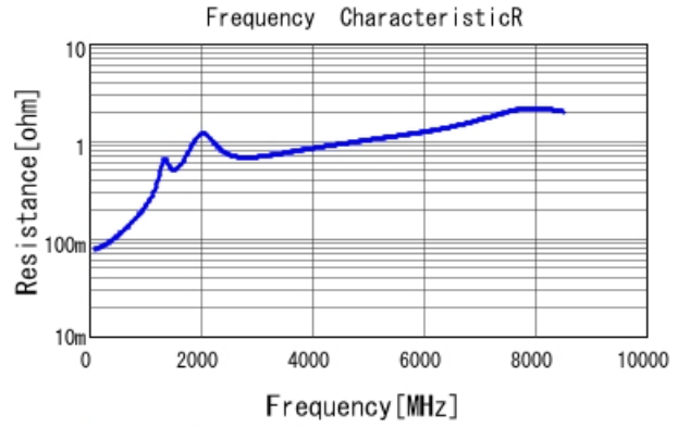
GRM1555C1H181JA01 R DCOV, 25degC
