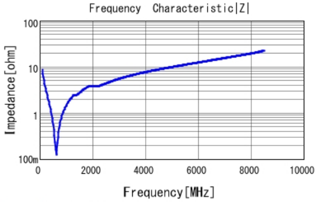
GRM1555C1H181GA01 |Z| DCOV, 25degC
