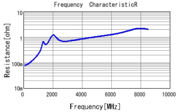
GRM1555C1H181GA01 R DCOV, 25degC
