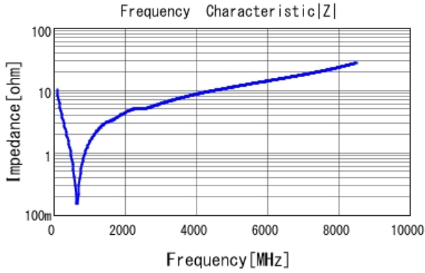
GRM1555C1H151GA01 |Z| DCOV, 25degC
