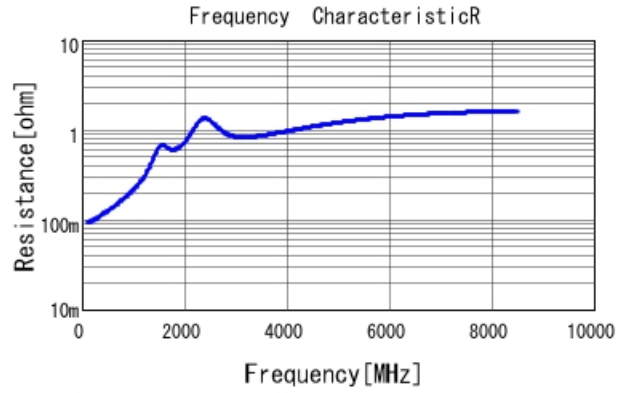
GRM1555C1H151GA01 R DCOV, 25degC
