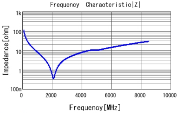
GRM1555C1H150JA01 |Z| DCOV, 25degC
