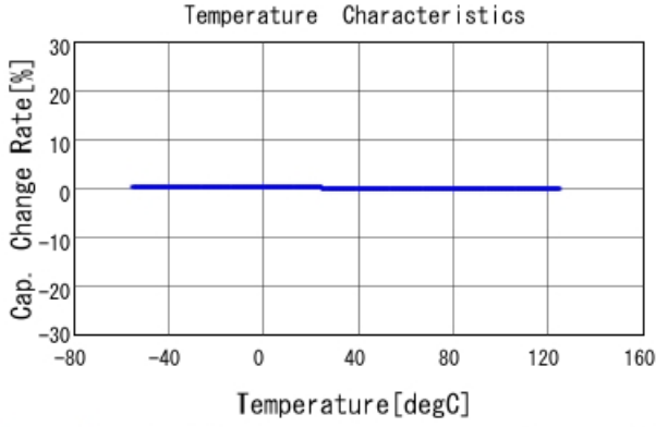
GRM1555C1H150JA01 C-Temp. capchange, DCOV, AC1Vrms
