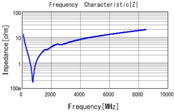
GRM1555C1H121JA01 |Z| DCOV, 25degC
