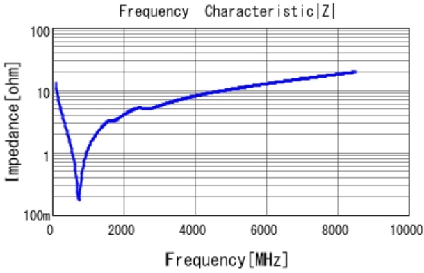
GRM1555C1H121GA01 |Z| DCOV, 25degC
