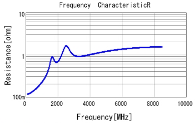
GRM1555C1H121GA01 R DCOV, 25degC
