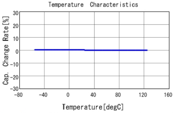
GRM1555C1H120JA01 C-Temp. capchange, DCOV, AC1Vrms
