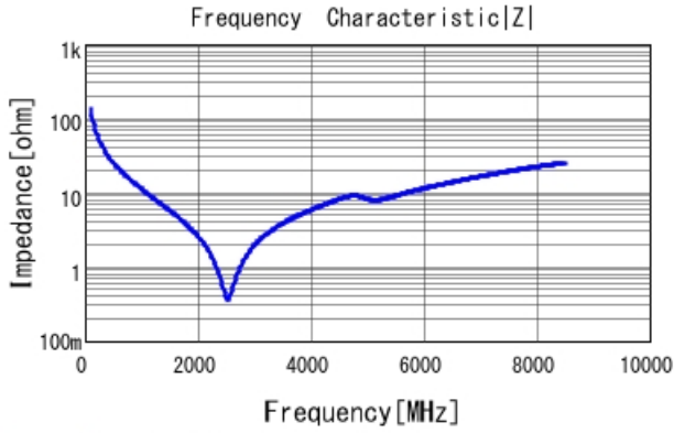
GRM1555C1H120JA01 |Z| DCOV, 25degC
