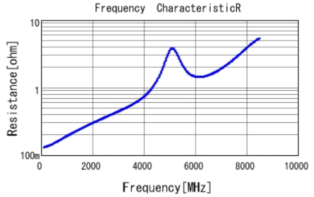
GRM1555C1H110JA01 R DCOV, 25degC
