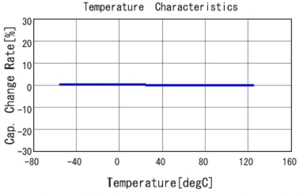
GRM1555C1H110JA01 C-Temp. capchange, DCOV, AC1Vrms
