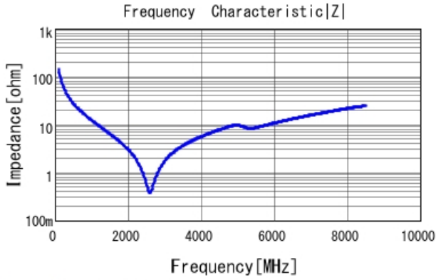
GRM1555C1H110JA01 |Z| DCOV, 25degC
