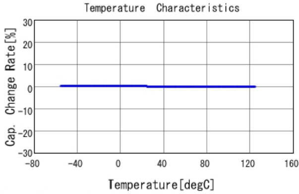
GRM1555C1H102JA01 C-Temp. capchange, DCOV, AC1Vrms
