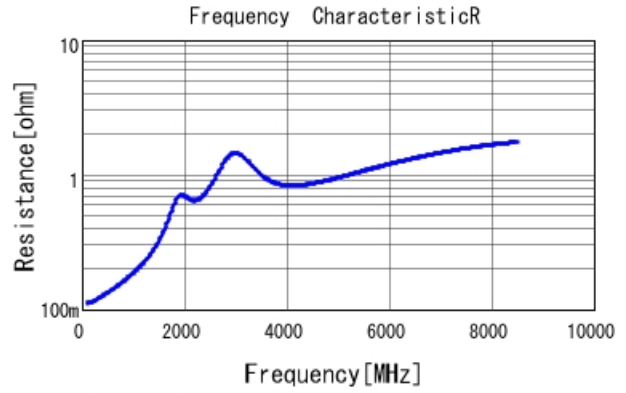
GRM1555C1H101JA01 R DCOV, 25degC
