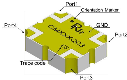
Figure 1. CMX21Q03 (Top View)
